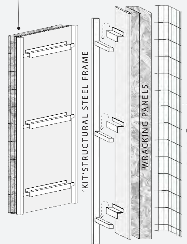
COPPER FIXINGS refer to Drawing set for material + structural performance + details
