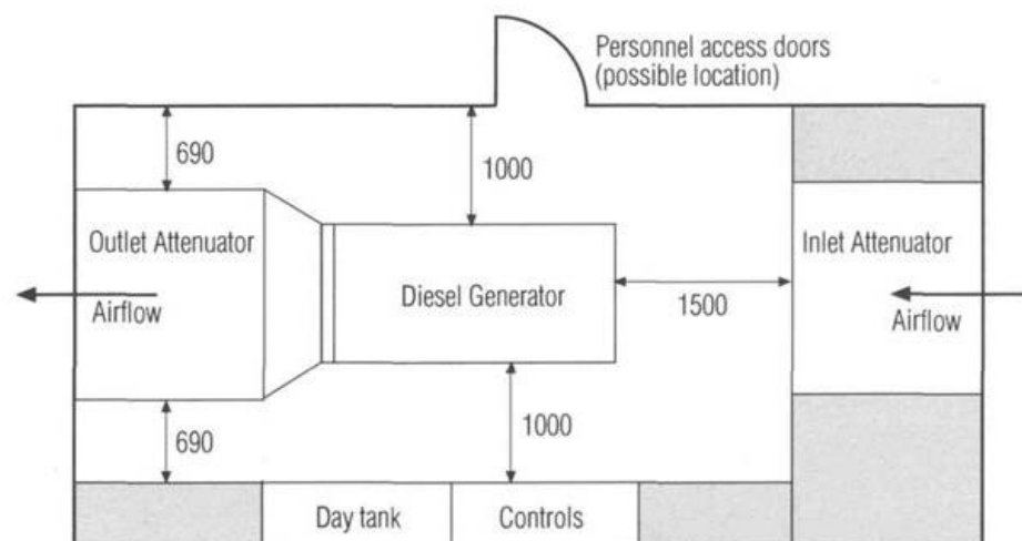
Figure 7.12 Diesel generating sets – Generator room with acoustic louvres
