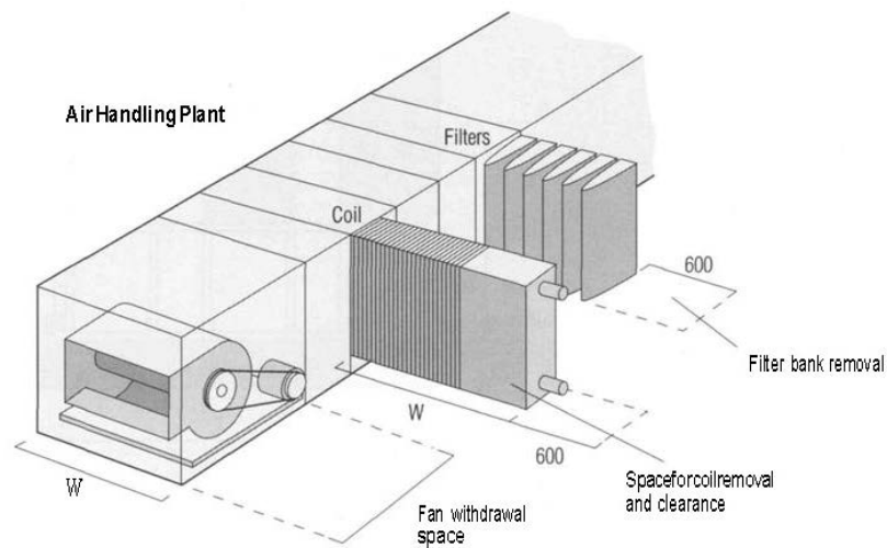
Figure 7.10 Air handling units space requirements
