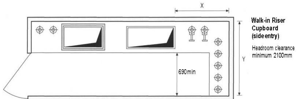
Figure 7.4 Mechanical risers
