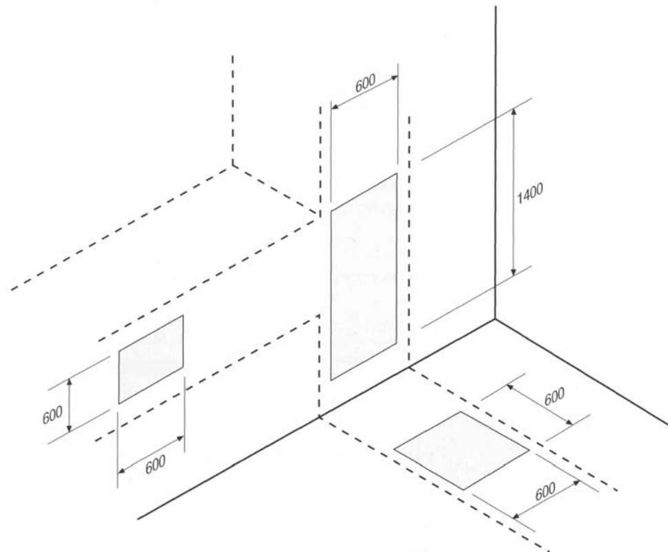
Figure 7.3 Access to distribution ducts and shafts
